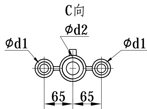
IME-03/BA外形尺寸
